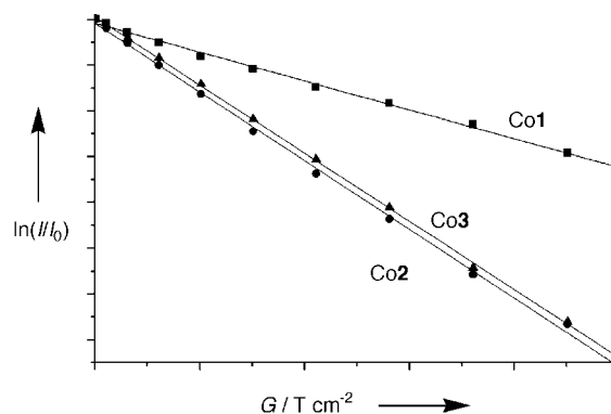
Figure 2. Variation in the intensity of the 1 H NMR signals of the aromatic protons of cobalt porphyrins (ln(I/I 0 )) in PGSE experiments, as a function of the field gradient (G). The measurements were carried out on a Bruker AMX-600 using 7 mM porphyrin solutions in chloroform/methanol (10/3).
